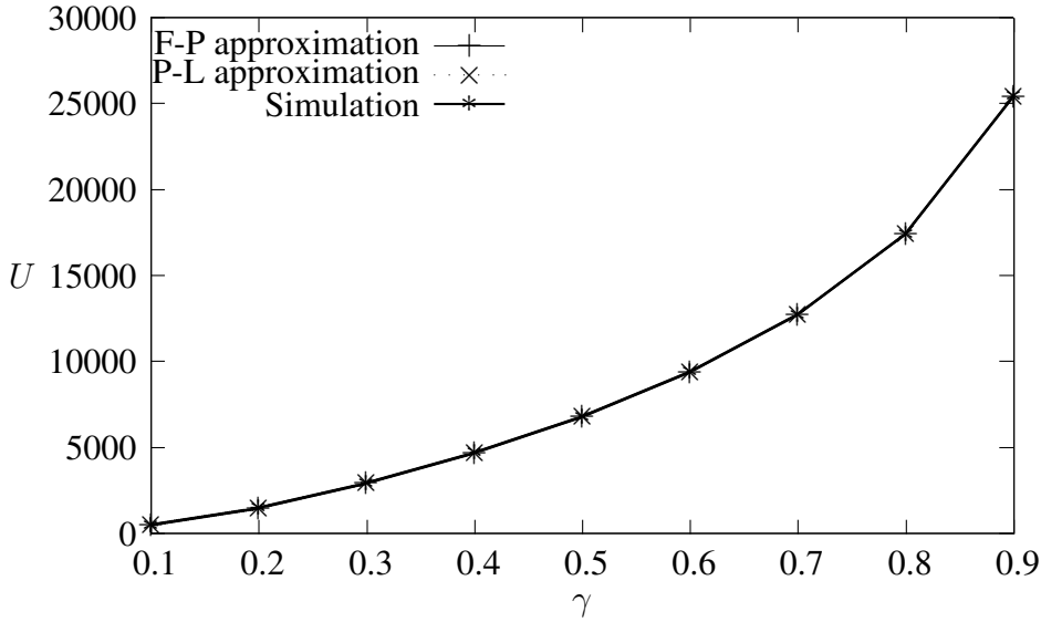
Figure 8. Large structured database: corruption time in days vs. fraction of corrupted edges.
