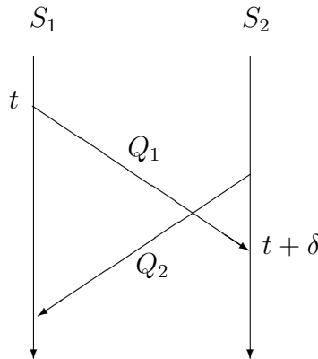
Figure 1. Conflict between Q_1 and Q_2 .
