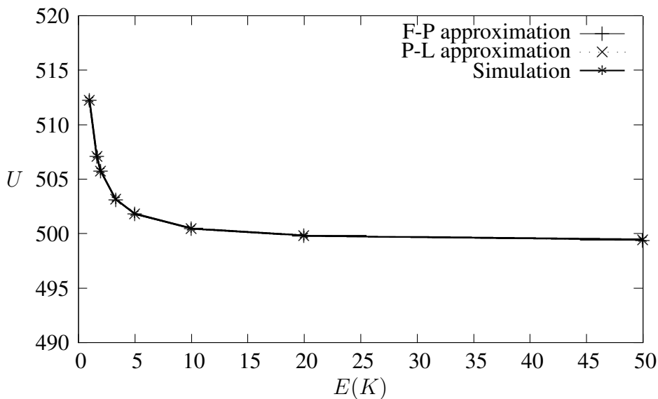
Figure 7. Large Structured Database: corruption time in days vs. average number of reads.
