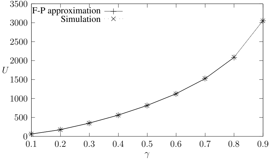
Figure 5. Varying fraction of corrupted edges.
