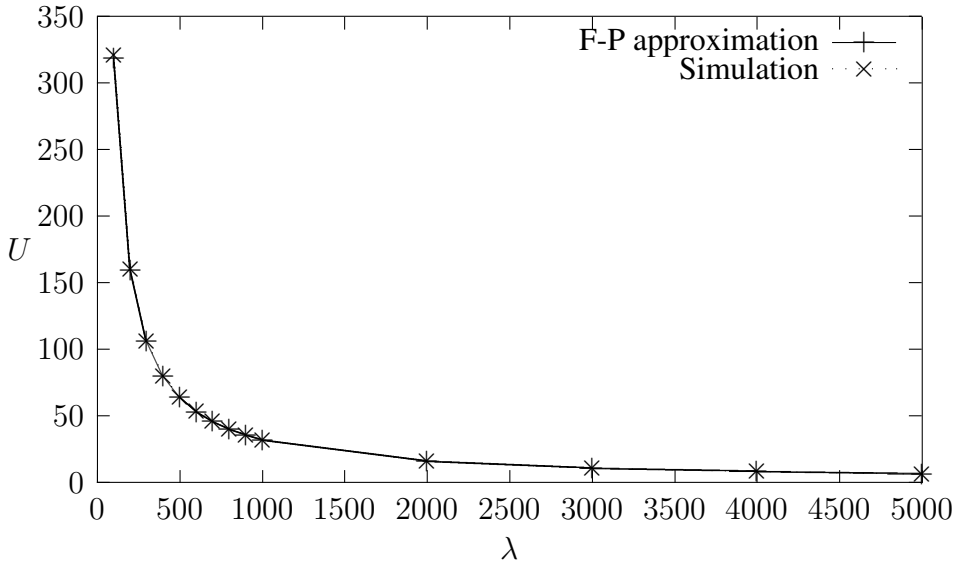
Figure 2. Corruption time in hours vs. arrival rate/sec.
