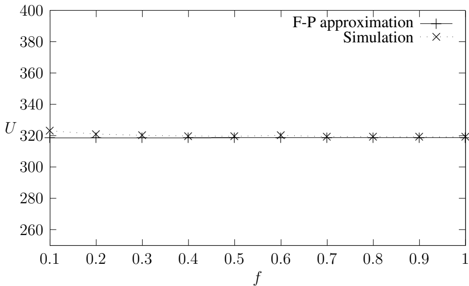
Figure 4. Varying fraction of distributed edges.
