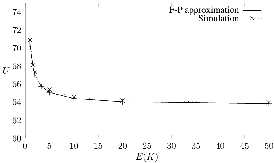
Figure 3. Corruption time in hours vs. average number of reads.
